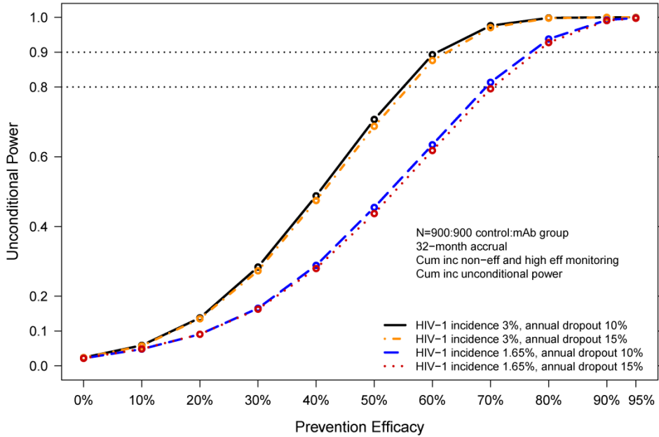
Figure 4-4 Unconditional power to reject H0: PE10 ≤ 0% in favor of H1: PE10 > 0% (or H0: PE30 ≤ 0% in favor of H1: PE30 > 0%) based on primary assumptions about HIV-1 incidence rate and dropout rate (1-sided 0.025-level tests). Power curves are also shown for lower than expected HIV-1 incidence rate and a higher than expected dropout rate.
