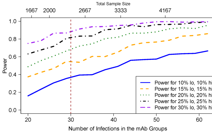
Figure 4-10 Power of the trial for detecting that PE varies over the three mAb marker-defined subgroups S(t) = Low, S(t) = Medium, and S(t) = High at level PE = 15%, 60%, 85%, respectively, for a marker with assay noise parameter rho = 0.9 and percentages of person-years at risk in the Low and High marker regions varied from 10%, 15%, 20%, 25%, 30%. The calculations at 2700 total participants assume 30 mAb group HIV-1-infected cases and 150 mAb group HIV-1-uninfected controls with data on S(t) and pool over both mAb groups.
