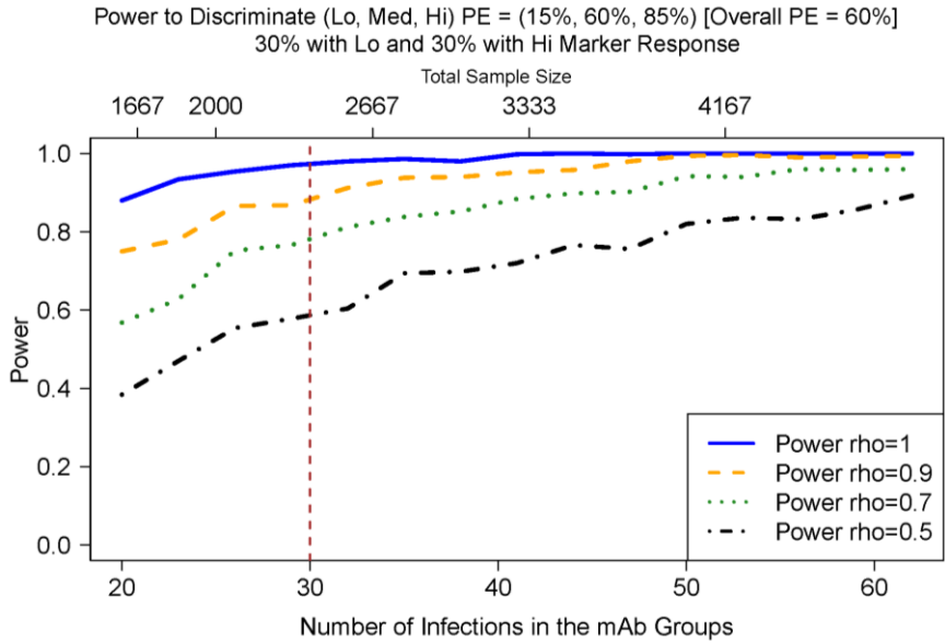
Figure 4-9 Power of the trial for detecting that PE varies over the three mAb marker-defined subgroups S(t) = \text{Low} , S(t) = \text{Medium} , and S(t) = \text{High} at level PE=15%, 60%, 85%, respectively, for a marker with assay noise parameter \rho = 1 (perfect marker), 0.9, 0.7, and 0.5 and percentages of person-years at risk in the (Low, Medium, High) marker regions set at (30%, 40%, 30%). The calculations at 2700 total participants assume 30 mAb group HIV-1–infected cases and 150 mAb group HIV-1–uninfected controls with data on S(t) and pool over both mAb groups. The dashed vertical line represents the sample size of the study.
