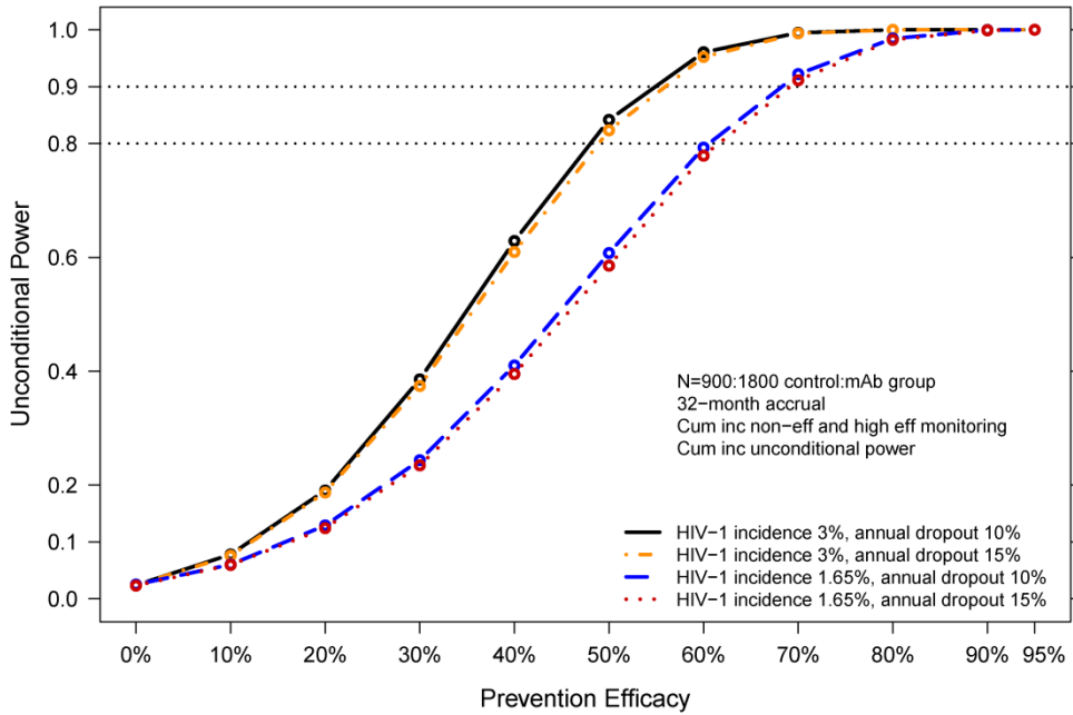
Figure 4-2 Unconditional power to reject H0: PE ≤ 0% in favor of H1: PE > 0% for a range of fixed values of pooled PE based on primary assumptions for HIV-1 incidence and dropout rate. Power curves are also shown for a lower than expected HIV-1 incidence rate and a higher than expected dropout rate.
