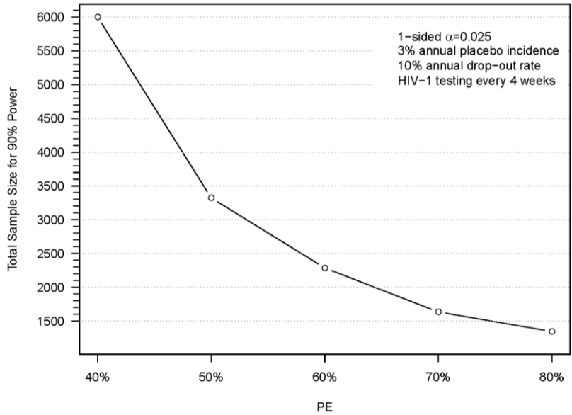
Figure 4-1 Total sample size for 90% power to reject H0: PE ≤ 0% in favor of H1: PE > 0% in a 1:1:1 allocation design with 80 weeks of follow-up for HIV-1 infection for each trial participant
